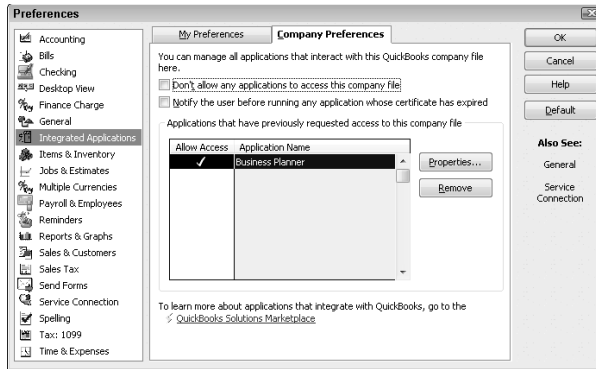
Figure 3-10: The Company Preferences tab of the Integrated Applications Preferences dialog box.
